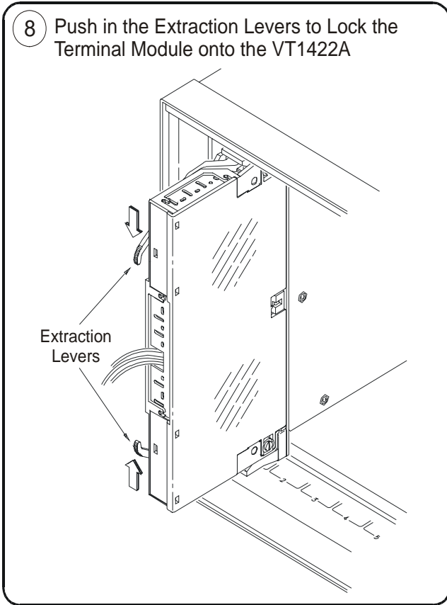
Figure 2-14. Closing and Attaching the VT1422A Terminal Module
