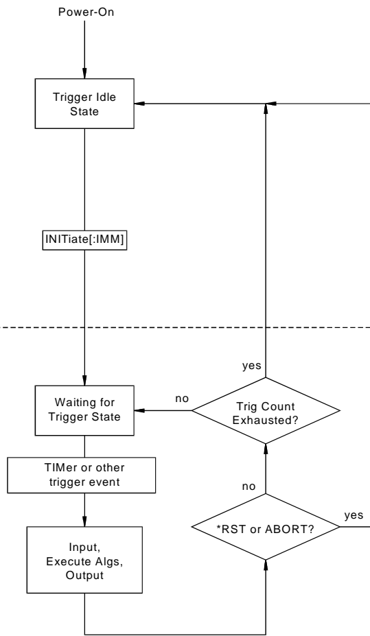
Figure 4-3. Module States
