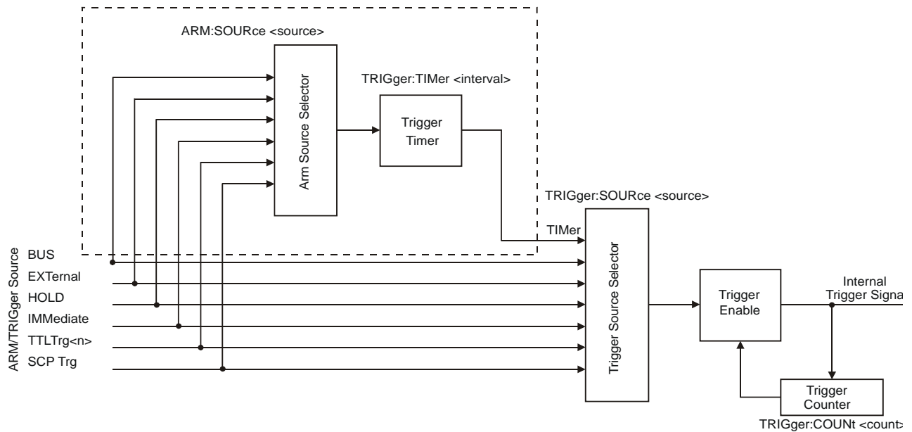
Figure 7-6. Logical Trigger Model
