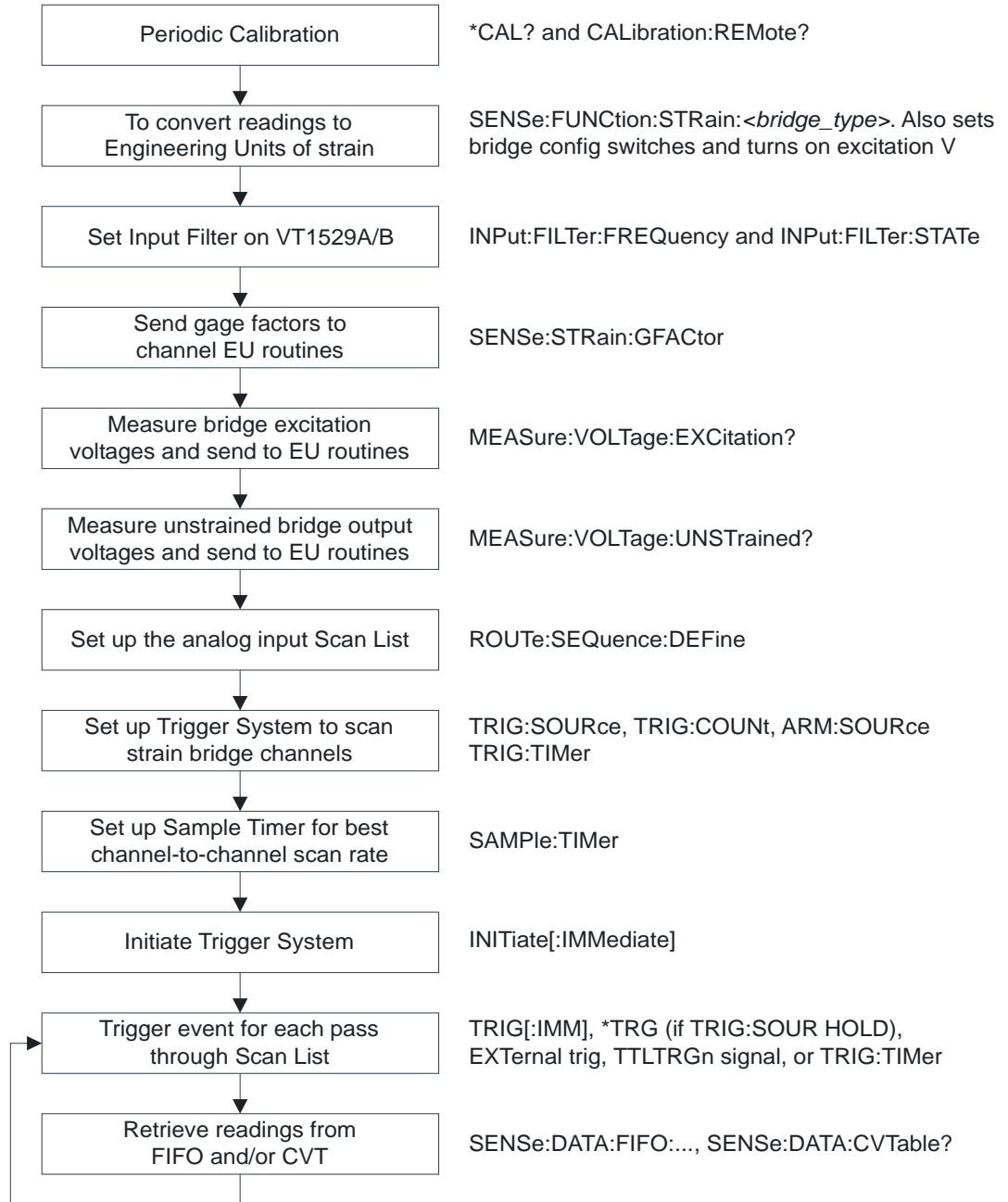
Figure 3-16. Sequence for Built-in Strain EU Conversion
